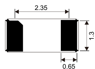
Pad Pattern
