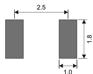
Pad Pattern
